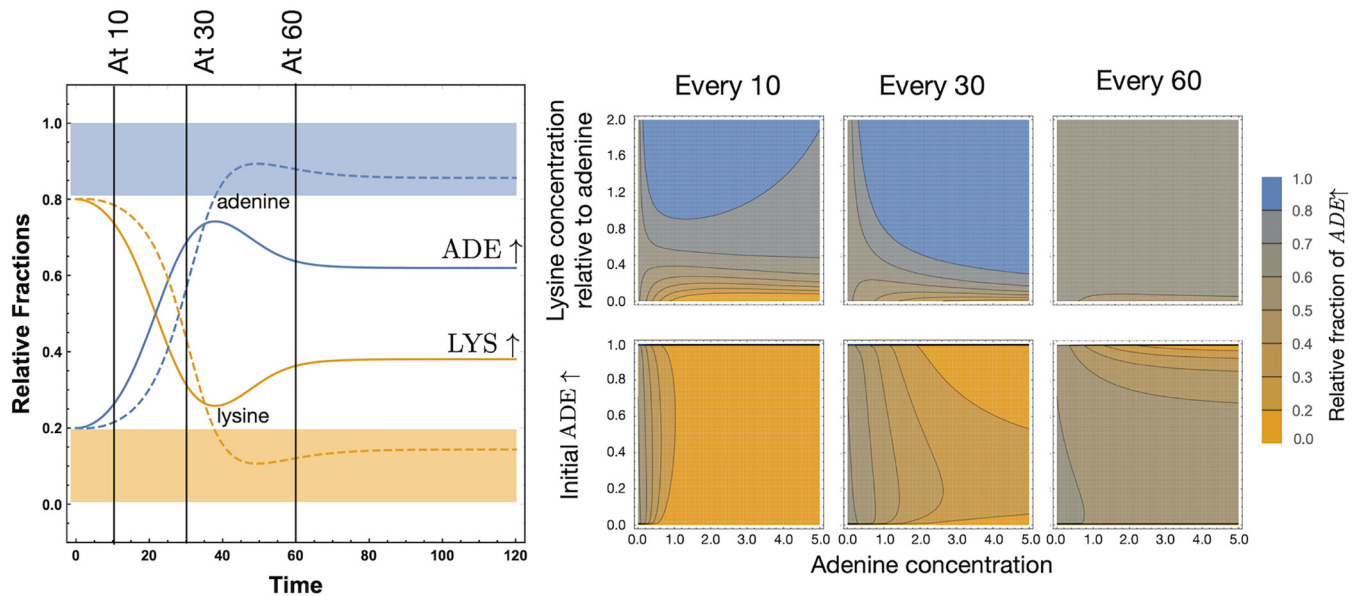
FIG 6 Disrupting transient mutualism with intermittent supplementation. Intermittent supplementation (Fig. 4) started with the same initial supplementation as the initial supplementation regime so as to be comparable. If we start with no metabolites in the culture and add them at fixed intervals, then it might be possible to maintain both mutualists at appreciable frequencies, even under supplementation. The exact timing of supplementation provided is crucial in determining the eventual equilibrium. If the pattern of supplementation starts early in the existence of the ADE ↑ strain, the resulting equilibrium frequency can be drastically affected. By tuning the timing and dose of supplementation, we can maximize the probability of maintaining the system close to the unsupplemented equilibrium state (as we move from supplementing every 10 to 30 to 60 time steps). If intermittent supplementation starts in the latter phase of the transient where the equilibrium value is already reached, the coexistence seems robust. This also depends on the initial concentration of the ADE ↑ strain (discussed further in the legend to Fig. 8). Thus, while the top row is calculated from an initial normalized concentration of 0.2 for the ADE ↑ strain, the bottom row explores all initial conditions. Equilibrium values are all calculated at the same time point, i.e., the number of cycles are adjusted so that all integrations run until the time point when cycle length × number of cycles = 300.
