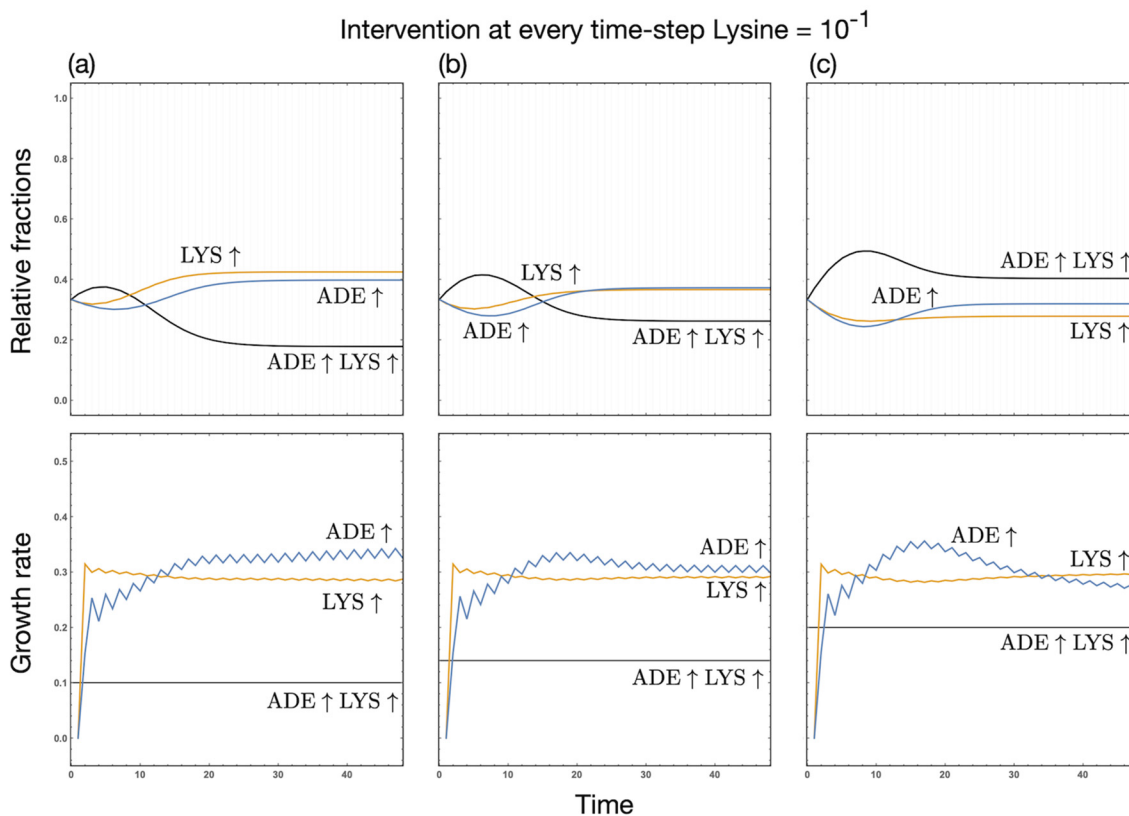
FIG 7 Ultimate overproducers and equilibrium dominance. By dominance we mean that one strain has a higher relative fraction in the culture. Here, we focus on intermittent supplementation which starts at a given time point and repeats after the same interval. For example, intervention at time point 2 starts supplementation at 2 and then every 2 time steps. The top grid panels show the dominant strain for a given intervention time and (Continued on next page)
