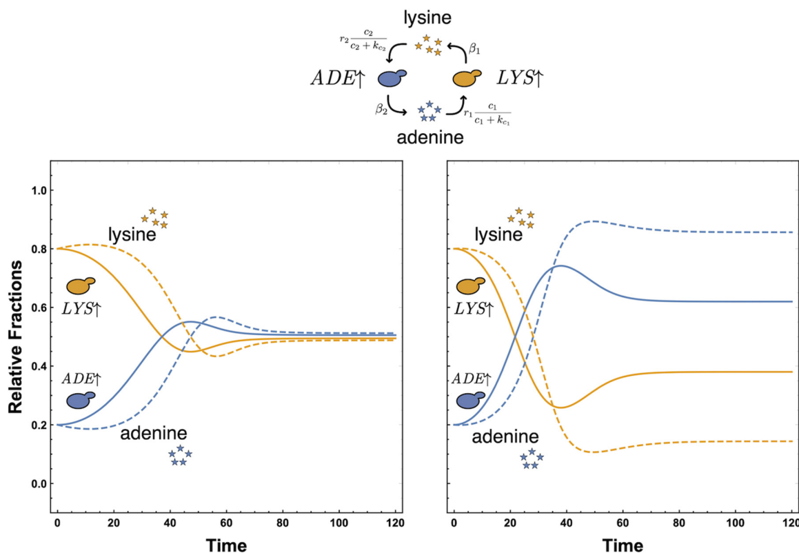
FIG 1 Theoretical model dynamics for the neutral expectation (left) and experimentally informed expectation (right). We plot the fractions of the LYS ↑ strain [ x_L/(x_L + x_A) ] and ADE ↑ strain [ x_A/(x_L + x_A) ] (solid lines) and the relative fractions of metabolites adenine [ c_A/(c_A + c_L) ] and lysine [ c_L/(c_A + c_L) ] (dashed lines) in a continuous culture. As an initial condition, there is no free adenine or lysine in the culture, but nonzero populations of the strains generate the free adenine and lysine in the same relative frequencies. The relative initial fractions for the strains are 0.8 for the LYS ↑ strain and 0.2 for the ADE ↑ strain, and the rate at which the two strains share the two metabolites is set to \beta_1 = \beta_2 = 0.1 . We set the carrying capacity of the culture vessel to K = 1 . (Left) The conversion rate of the metabolites to growth and the rate at which the metabolites are consumed are exactly the same ( r_1 = r_2 = 1 and \gamma_1 = \gamma_2 = 1 ). The Michaelis constant for both metabolites to k_{c_A} = k_{c_L} = 1 . Under these symmetric conditions, the relative fractions of the strains, as well as those of the two metabolites, reach an equilibrium where normalized concentrations are the same. (Right) Clearly, the symmetry assumption in all the rates is a simplification. Informed by experiments, we estimate that the growth constant of the ADE ↑ strain to be twice as much as of the LYS ↑ strain, r_1 = 1 , r_2 = 2 , and the Michaelis constants k_{c_A} = 2 and k_{c_L} = 1 . This asymmetry in uptake rates is reflected in the resulting unequal equilibrium.
