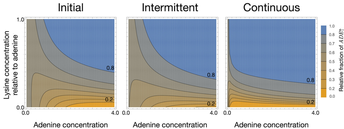
FIG 4 Equilibrium value of the ADE \uparrow strain for different supplementation regimes. The initial normalized concentration of the ADE \uparrow strain was 0.5. The system is assumed to have equilibrated when values of the strain densities do not change more than 10^{-4} between two consecutive numerical time steps. By 300 time steps, all initial conditions for initial supplementation have already reached this equilibrium state, and hence, we choose to show the snapshot of the system at time point 300. In the plots, we show the eventual normalized concentration of the ADE \uparrow strain going from all ADE \uparrow strain (relative fraction value of 1, blue) to all LYS \uparrow strain (relative fraction value of 0, yellow). In each plot, the initial concentration of adenine in the system at time zero is shown on the x axis, and the amount of lysine relative to adenine is depicted on the y axis. For y = 1 , the amounts of adenine and lysine are the same. In initial supplementation, metabolites were provided only at time point t = 0 . In intermittent supplementation, metabolites were provided starting at t = 25 and then every 25th time step. For continuous supplementation, metabolites were provided at every time step. Going from initial to continuous supplementation, we see that the zone (between contours 0.2 and 0.8) shrinks as the zone for the LYS \uparrow strain (yellow) increases, and so does the ADE \uparrow strain (blue) region.
